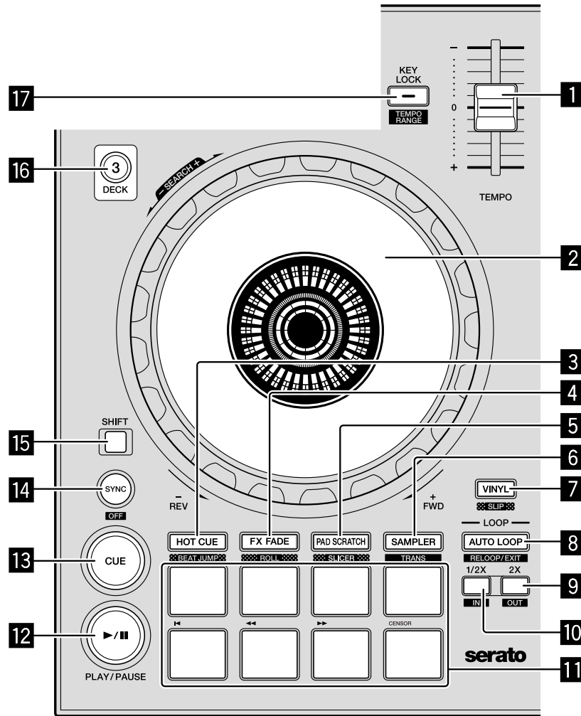
Fig. 56: Deck section (p. 6)
